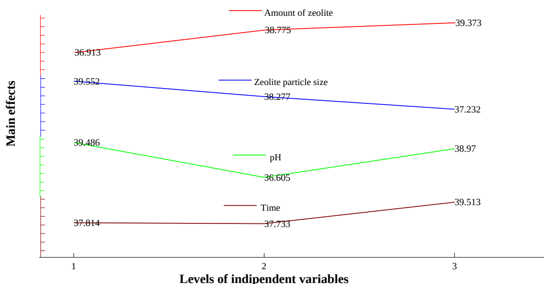
Fig. 4. The main effects of particle size; time; amount of zeolite and pH on arsenic removal by \text{FeCl}_3 \cdot 6\text{H}_2\text{O} modified zeolite from aqueous solution.
