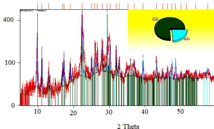
Fig. 1. XRD results of natural Sabzevar zeolite powder.
