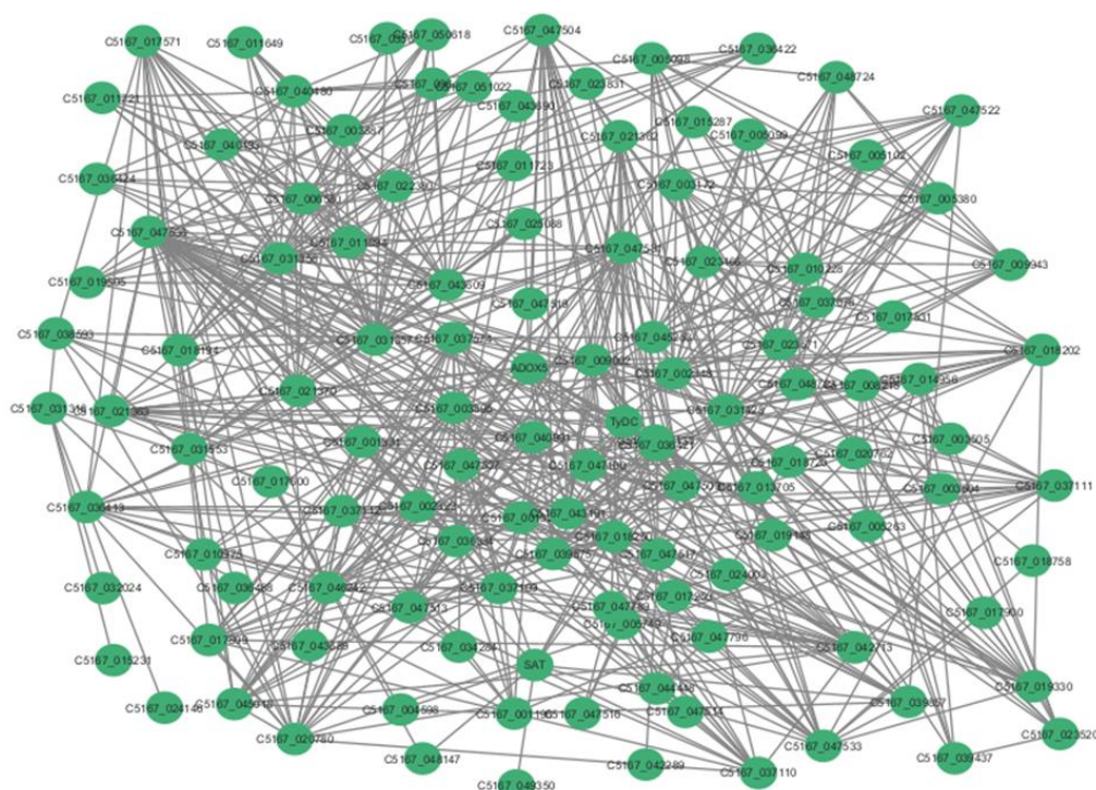
Figure 1. PPI Network of the morphine biosynthesis genes in opium poppy using Cytoscape software and STRING database (Genes related to morphine biosynthesis were first placed in the String database and then transferred to Cytoscape software to examine the relationships of these genes).
