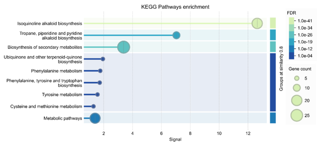
Figure 3. Kyoto Encyclopedia of Genes and Genomes (KEGG) pathways analysis on the hub genes in morphine biosynthesis using STRING version10. ( In this analysis, Isoquinoline, Tropen, piperidine and pyridine alkaloid biosynthesis, Biosynthesis of secondary metabolites, Ubiquinone and another terpenoid-quinone biosynthesis, phenylalanine metabolism, Phenylalanine, tyrosine and tryptophan biosynthesis, Tyrosine metabolism, Cysteine and methionine metabolism, Metabolic pathways play a role).
