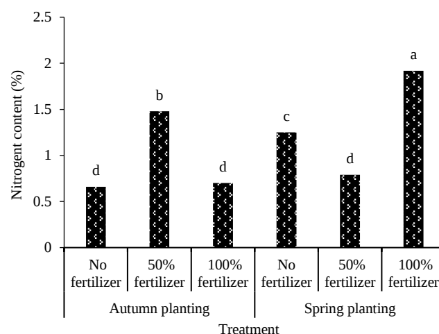
Figure 2. The effects of planting date and the amount of nitrogen and phosphorus fertilizers on seed nitrogen percentage. Means with the same letter are not significantly different according to Duncan's test at P = 0.05 .
