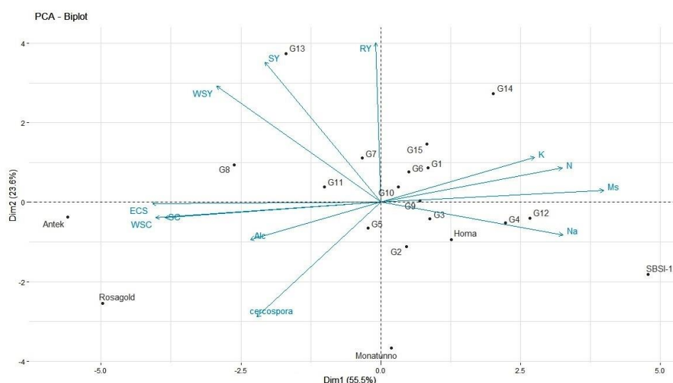
Figure 3. Scatter biplot diagram of sugar beet genotypes based on the first and second components in Dezful
