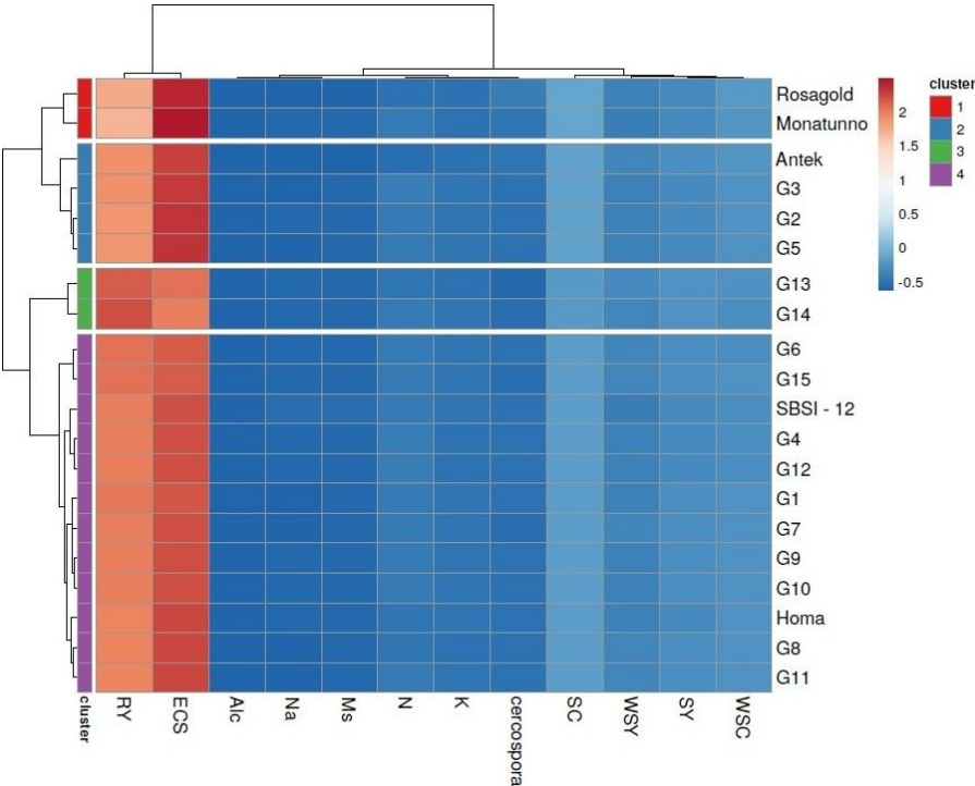
Figure 1. Heat map dendrogram of cluster analysis for sugar beet genotypes and their quantitative and qualitative characteristics in Dezful
