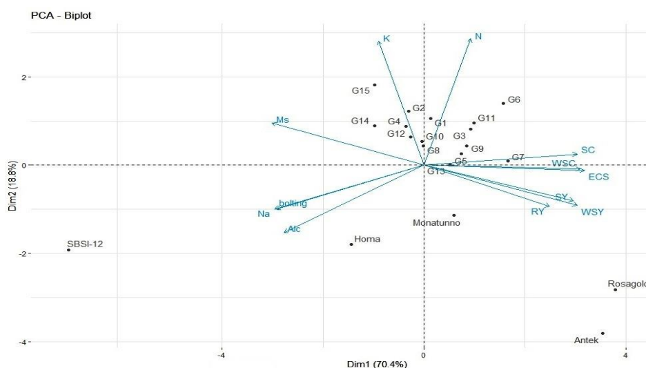
Figure 4. Scatter biplot diagram of sugar beet genotypes based on the first and second components in Gachsaran
