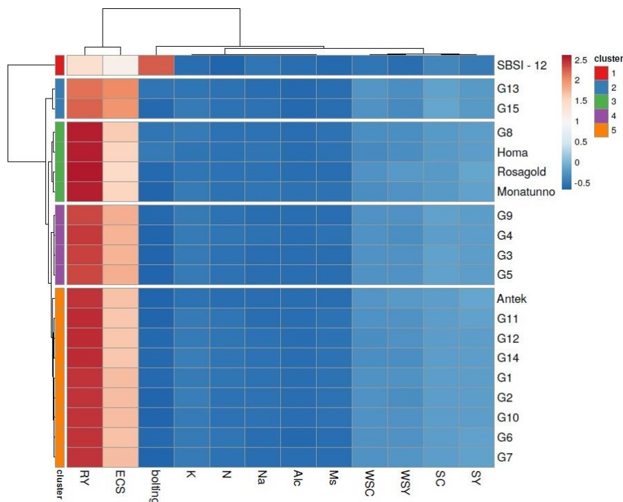
Figure 2. Heat map dendrogram of cluster analysis for sugar beet genotypes and their quantitative and qualitative characteristics in Gachsaran
