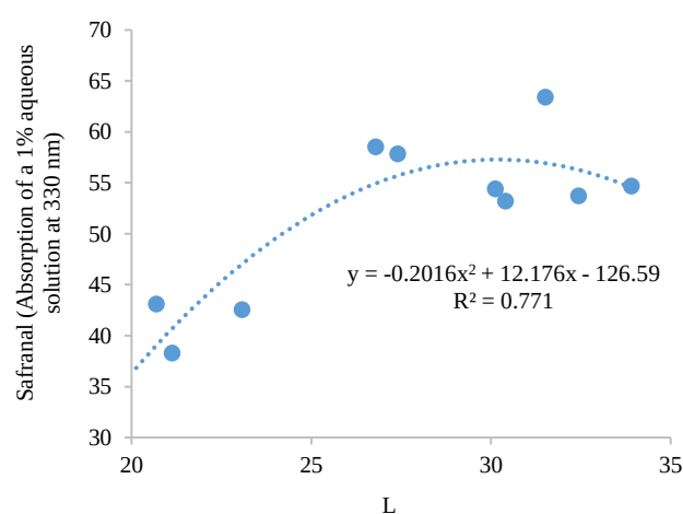
Figure 4. Regression relationship between safranal and L index in saffron stigma.
