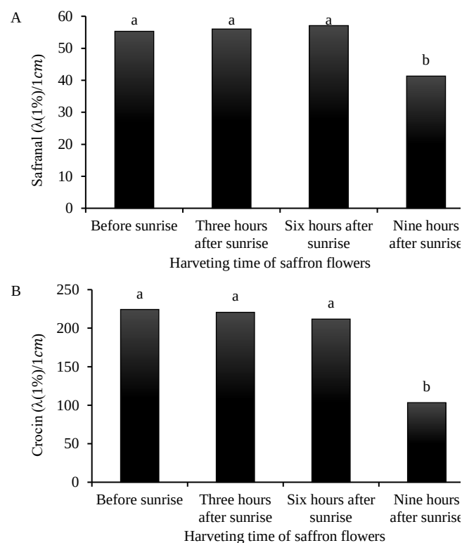
Figure 3. Effect of harvesting time of saffron flowers during the day on safranal (A) and crocin (B) content of stigma (the units are absorbance of 1% aqueous stigma extract at 330 nm for safranal and 440 nm for crocin).
